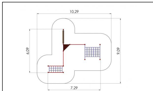
TKR001-4 - Balance Model 4
