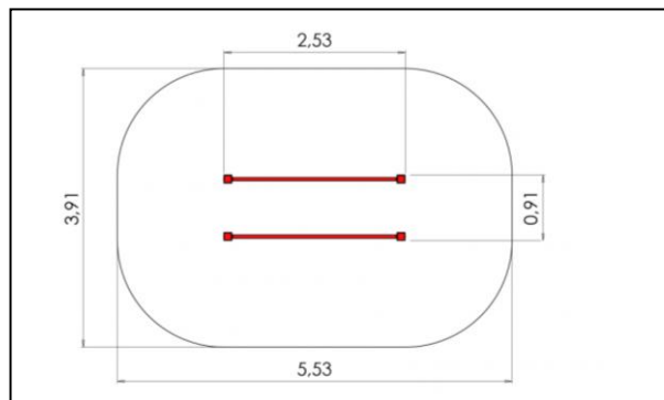
TSV003 - Push-up bars
