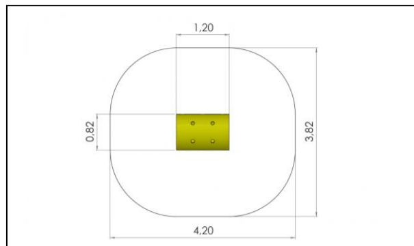
PVP10 - Spiral balance SNAKE
