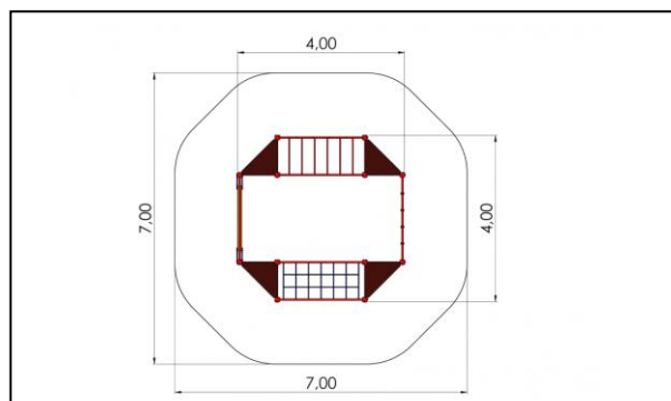
TKR001-5 - Balance Model 5
