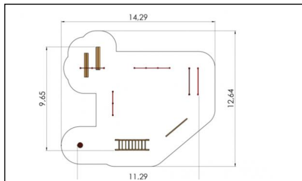
TSV011 - Outdoor exercise complex 2
