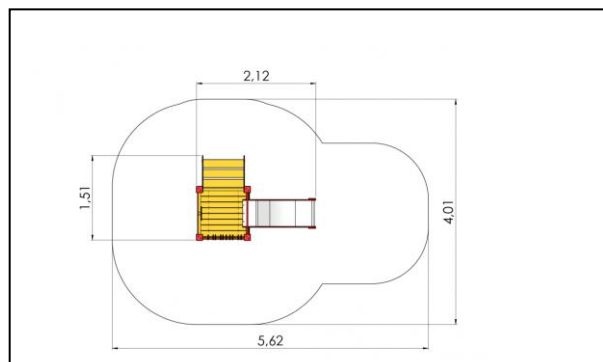
LM001 - Slide TIM
