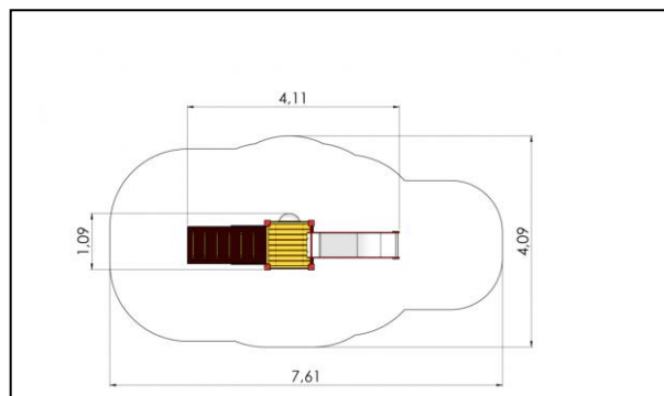
LM002PE - Slide ANN
