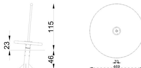
NO.03 Three hangar caroussel
