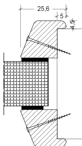
62mm BD60 glas
