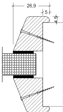
62mm BD30 glas
